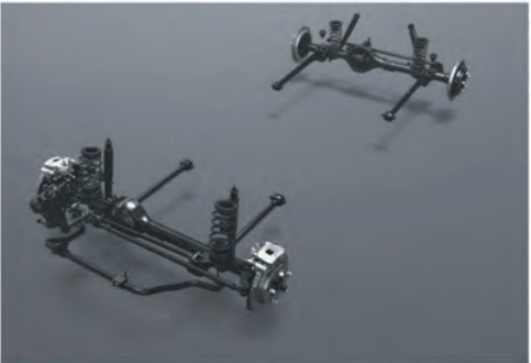
3 LINK RIGID AXLE SUSPENSION
